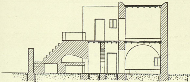
ΤΟΜΗ Α.Α'.Β.Β'
